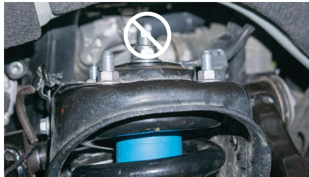
Fig. 7: Remove the four top hat nuts.
