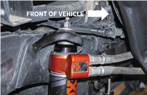
Fig. 21: Install the stem top nut (passenger side shown).
