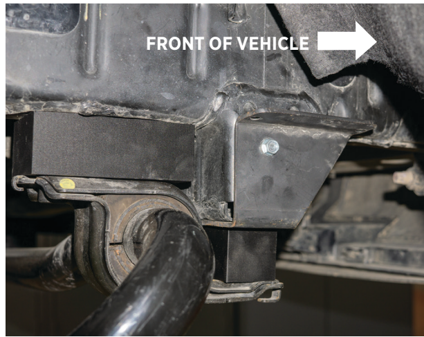
Fig. 6: Install the reservoir bracket assembly.
