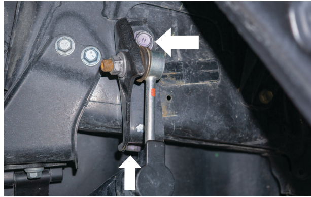
Fig. 25: Remove the two sway bar bracket bolts (passenger side shown).
