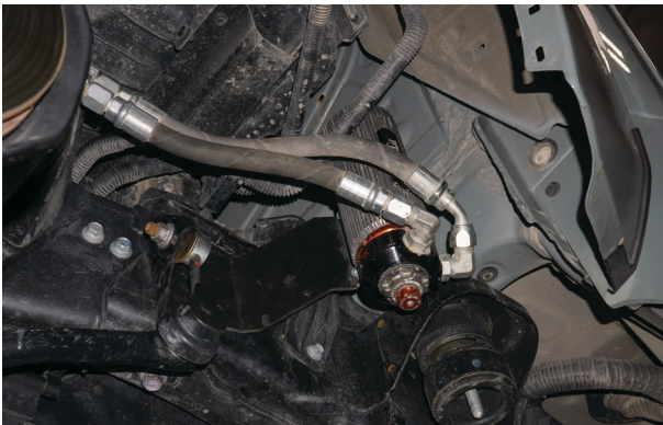
Fig. 26: Install the reservoir (passenger side shown).
