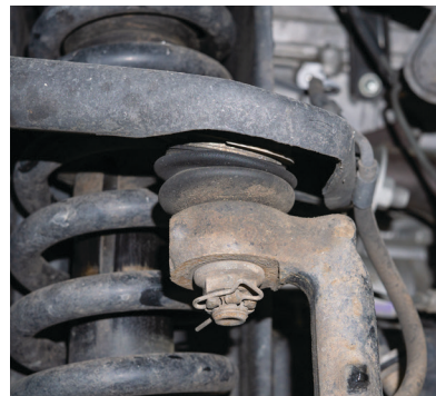
Fig. 3: Disconnect UCA.
