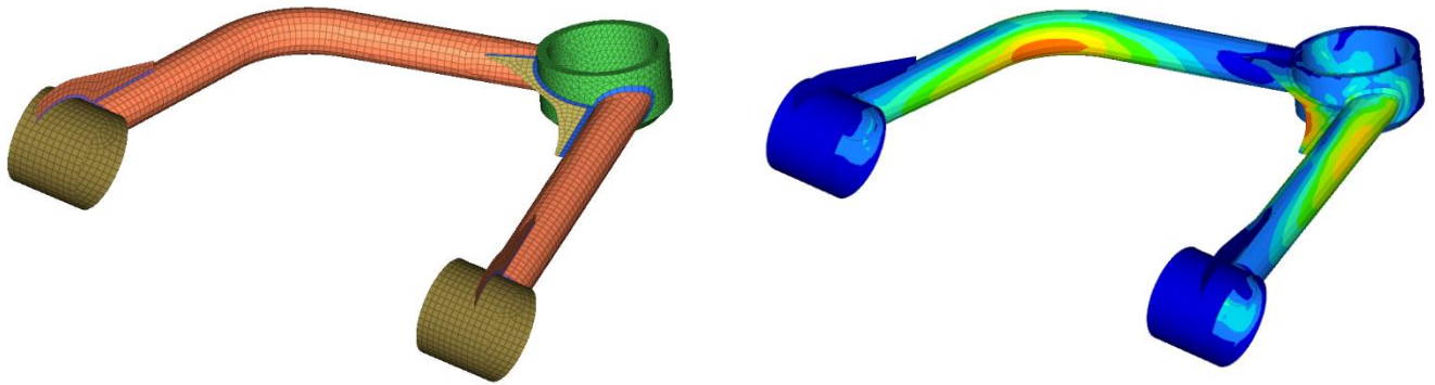
Figure 2: Upper Control Arm Mesh and Stress Contour
