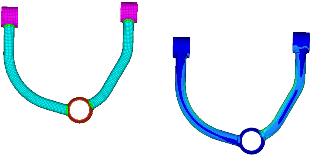
Figure 2: Upper Control Arm Mesh and Stress Contour
